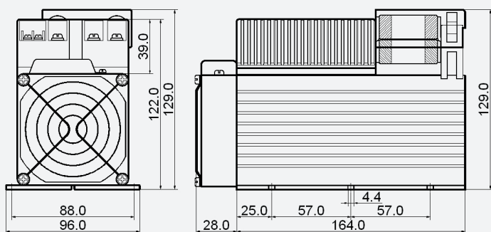
ESR-xxDA+ / ESR-xxDA-H+
