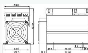
LSR-F-40/60/80/100/+Fuse+Fan
