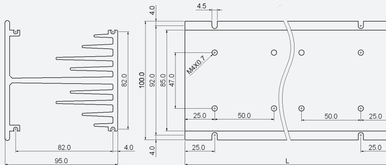
Standard type
