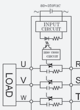
TSR-25AA-□ / TSR-40AA-□
