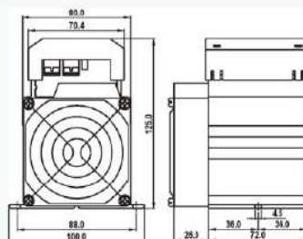
ASR-F-60/80/100/ACR-F-60/80/100+ Fan
