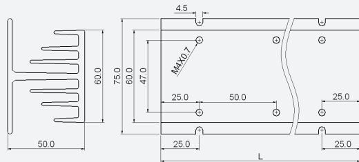
H type
