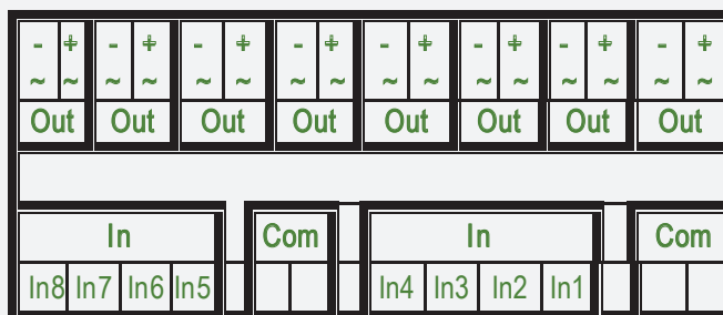
SSR-P03□-8P
