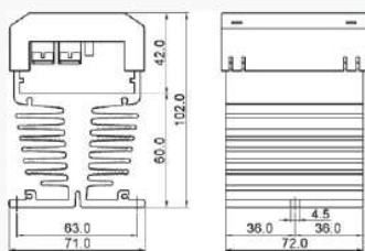
ASR-40 / ACR-40
