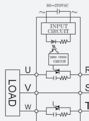
TSR-50AA-□ / TSR-75AA-□
