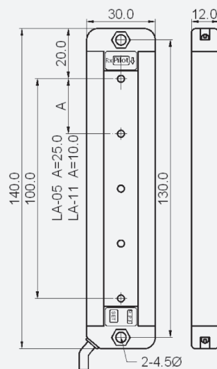
Receiver (Rx)
