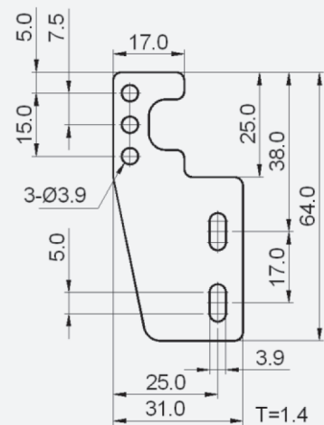
Bracket
