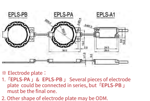
EPLS-A1N+ EPLS-PA + EPLS-PB
