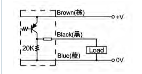
PNP
